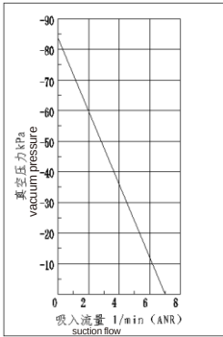
流量特性:flow characteristic
