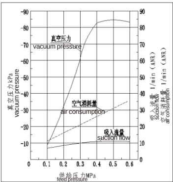
排气特性:Exhaust characteristic
